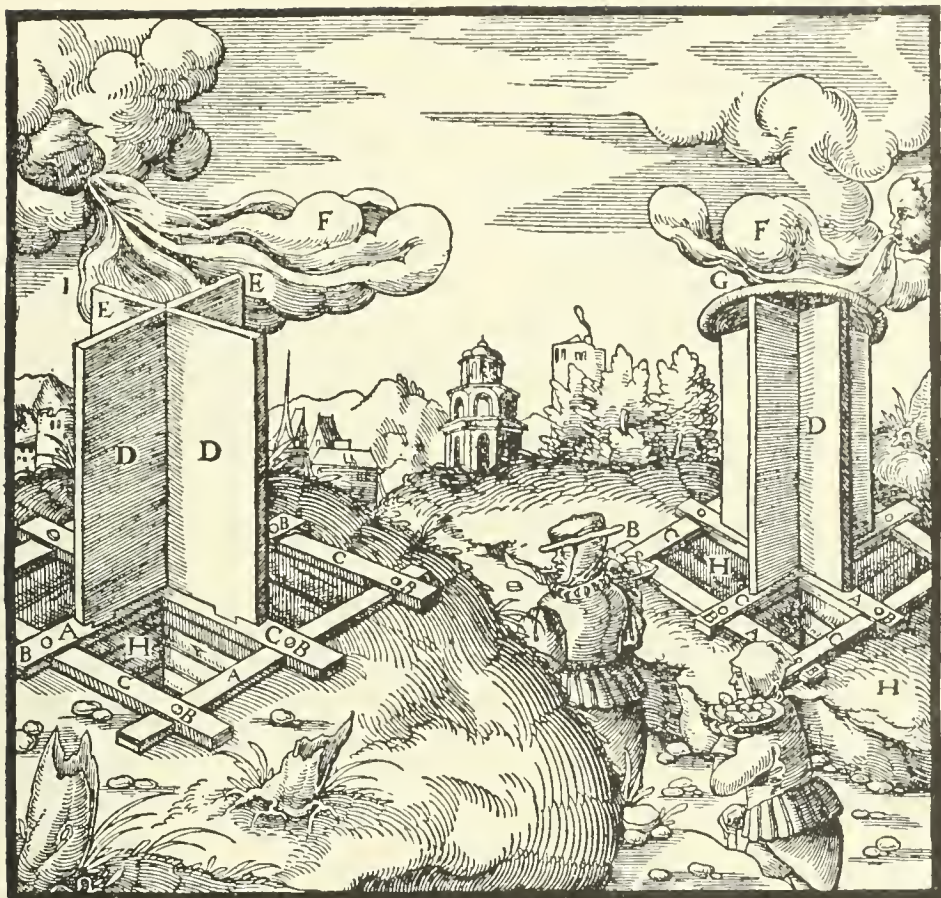
A—SILLS. B—POINTED STAKES. C—CROSS-BEAMS. D—UPRIGHT PLANKS. E—HOLLOW. F—WINDS. G—COVERING DISC. H—SHAFTS. I—MACHINE WITHOUT A COVERING.
